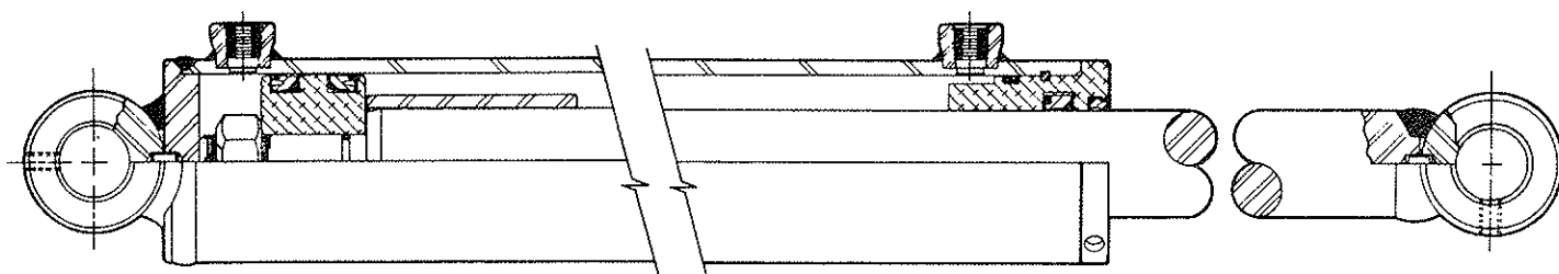
BOOM EXTEND CYLINDER
